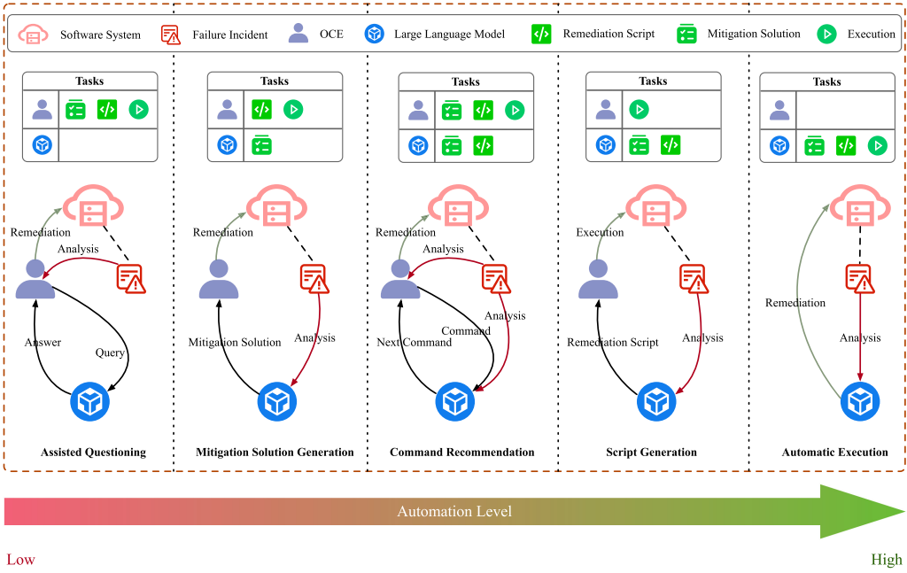
Fig. 9. Various Types of Auto Remediation Approaches.
